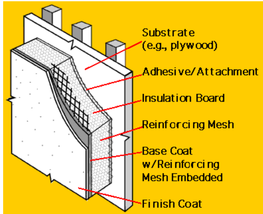
EIFS System Components
